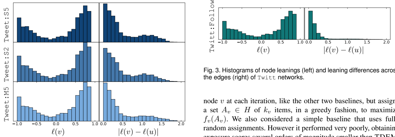
Fig. 2. Histograms of node leanings (left) and leaning differences across the edges (right) of Tweet networks.
