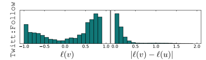
Fig. 3. Histograms of node leanings (left) and leaning differences across the edges (right) of Twitt networks.
